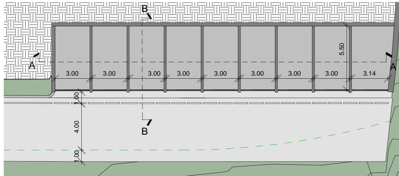
PLANIMETRIA PIANO BOX
